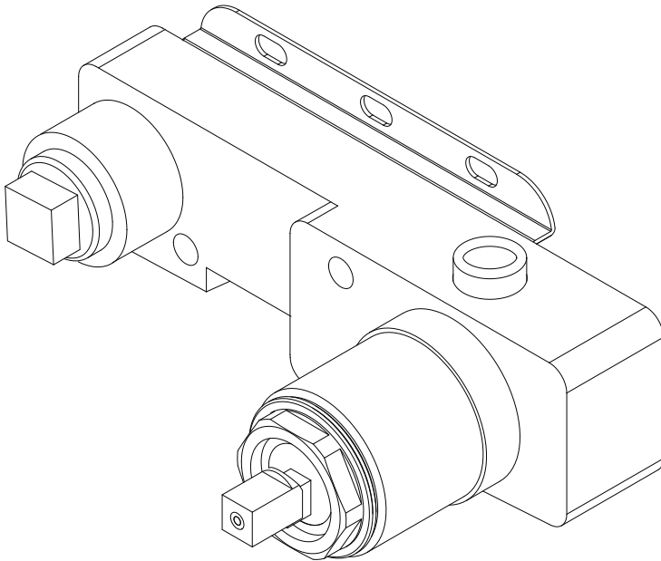
3D View Vista Tridimensional
